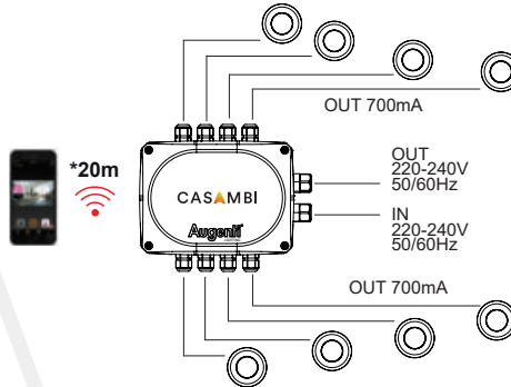
RIM45 HUB.700.001.CA 700mA CASAMBI MAX 8 pz.
