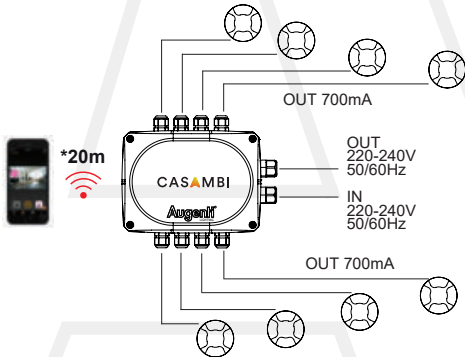
CUT45 HUB.700.001.CA 700mA CASAMBI MAX 8 pz.
